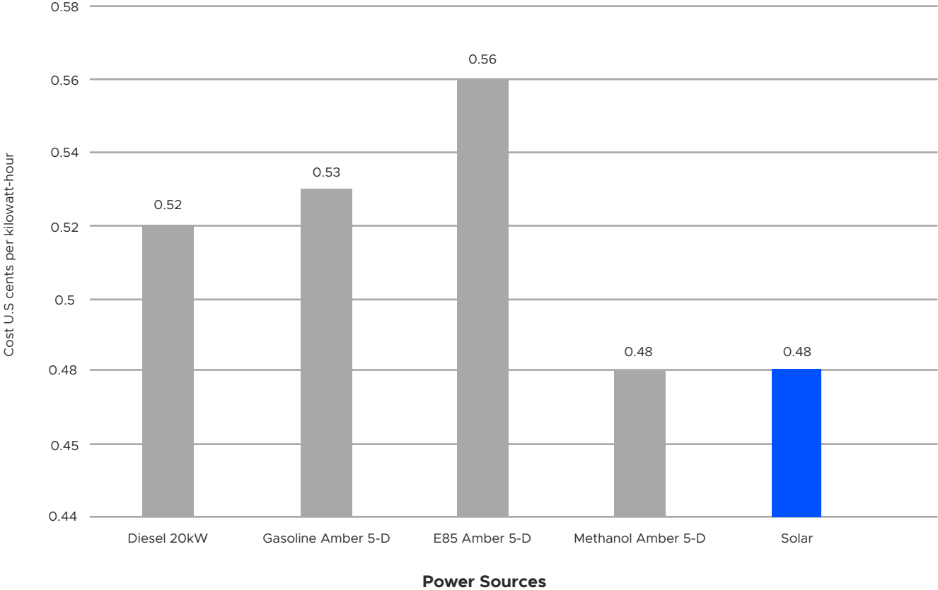
Average renewable electricity generation cost worldwide in 2021, by energy source
